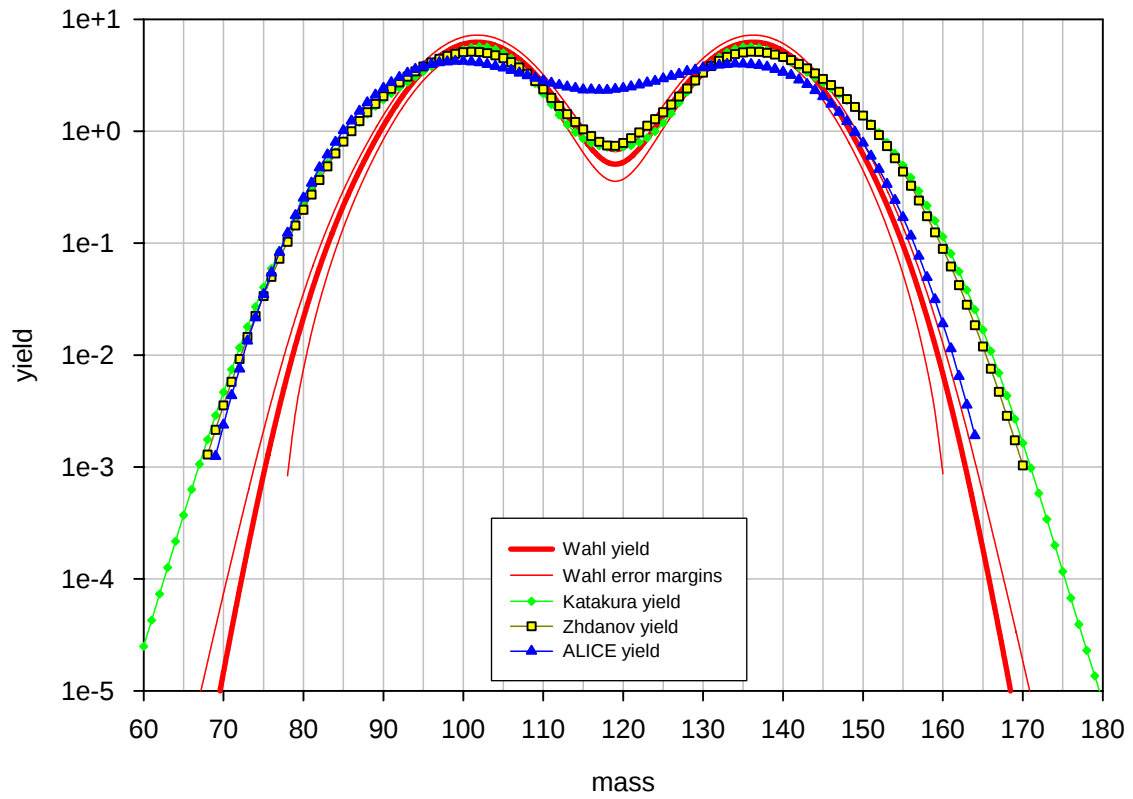
Benchmark B: ^{241}\text{Am} at 13 MeV, post neutron emission yield
